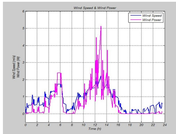
Fig. 8 . The comparison between wind speed and energy produced by wind turbine
