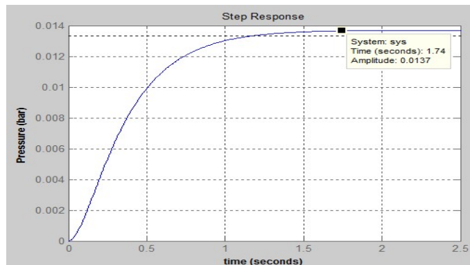
Fig. 3 . Step response of system
