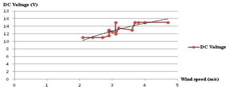
Fig. 15 . Graph showing relations between DC voltage and wind speed
