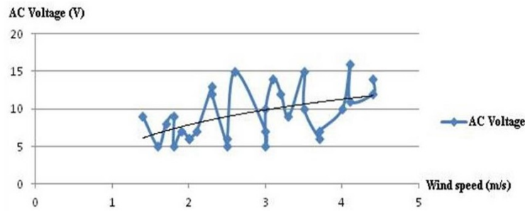
Fig. 14 . Graph showing relations between generated AC electricity voltage and wind speed.
