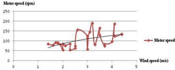
Fig. 13 . Graph showing relations between a rotational speed of an electric bicycle motor and wind speed
